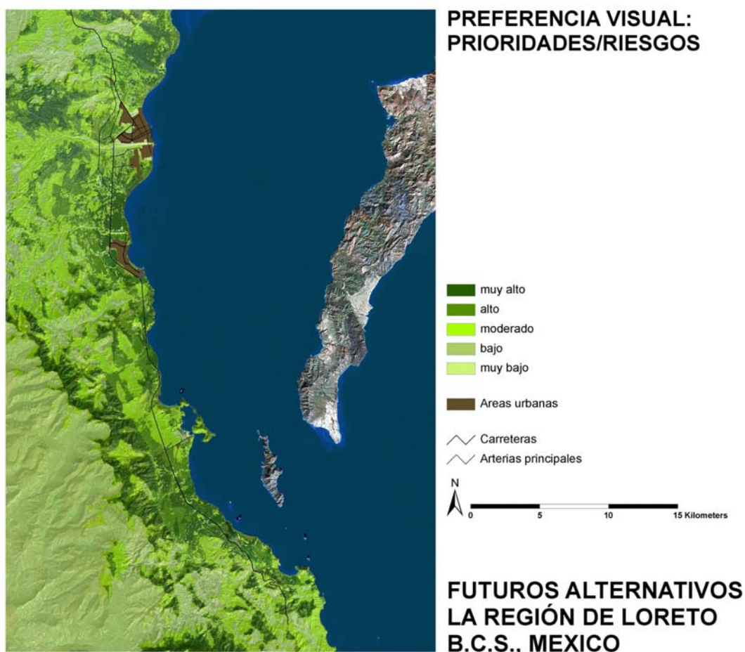
Figure 20. View Preferences
